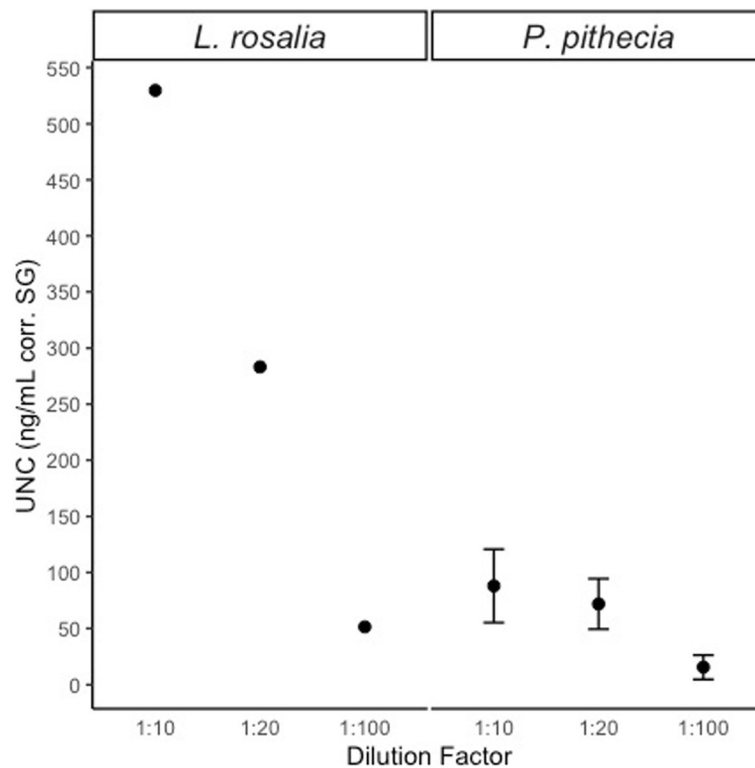
Fig. 1 Measures of UNC in samples collected from captive Leontopithecus rosalia ( n = 1) and Pithecia pithecia ( n = 5) diluted to three dilution factors. Samples were diluted in assay buffer and ran in duplicate. Data shown for P. pithecia is average \pm standard deviation. No error bars are shown for L. rosalia as there was only one sample included for this analysis
