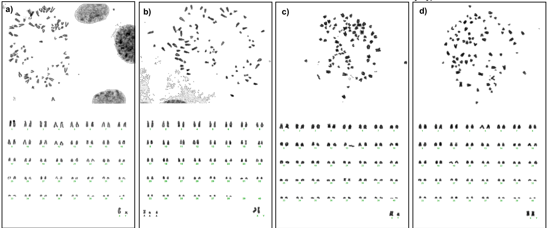
Supplementary Figure 5: a) Karyotype and metaphase spread of representative fibroblasts of a male NWR, KB 9947 b) Karyotype and metaphase spread of fibroblasts from a female 2n = 81 NWR, KB 8173 c): Representative karyotype and metaphase spread of reprogrammed iPSCs of a male 2n = 82 NWR, 5765-c509 d) Representative karyotype and metaphase spread of reprogrammed iPSCs of a female 2n = 82 NWR, 17626-c5103. All karyotypes show the expected chromosome complement.
